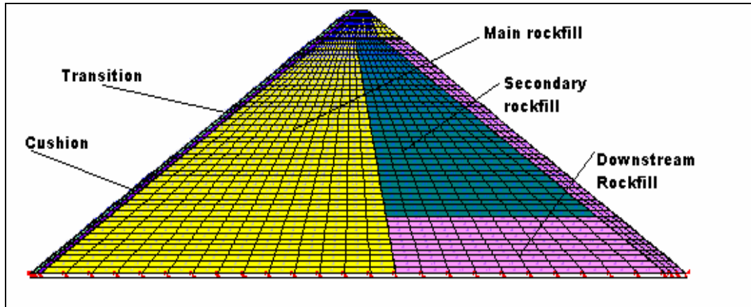
Figure 2: Shibuya Dam, FEM mesh and dam zoning.
