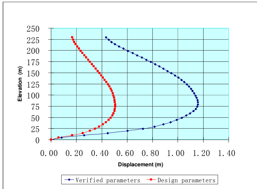
Figure 8: Calculated settlements (m) at the end of the filling of the reservoir for a CFRD
