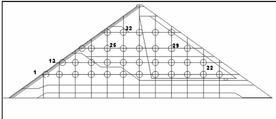
Figure 4: Location of the monitored points.
