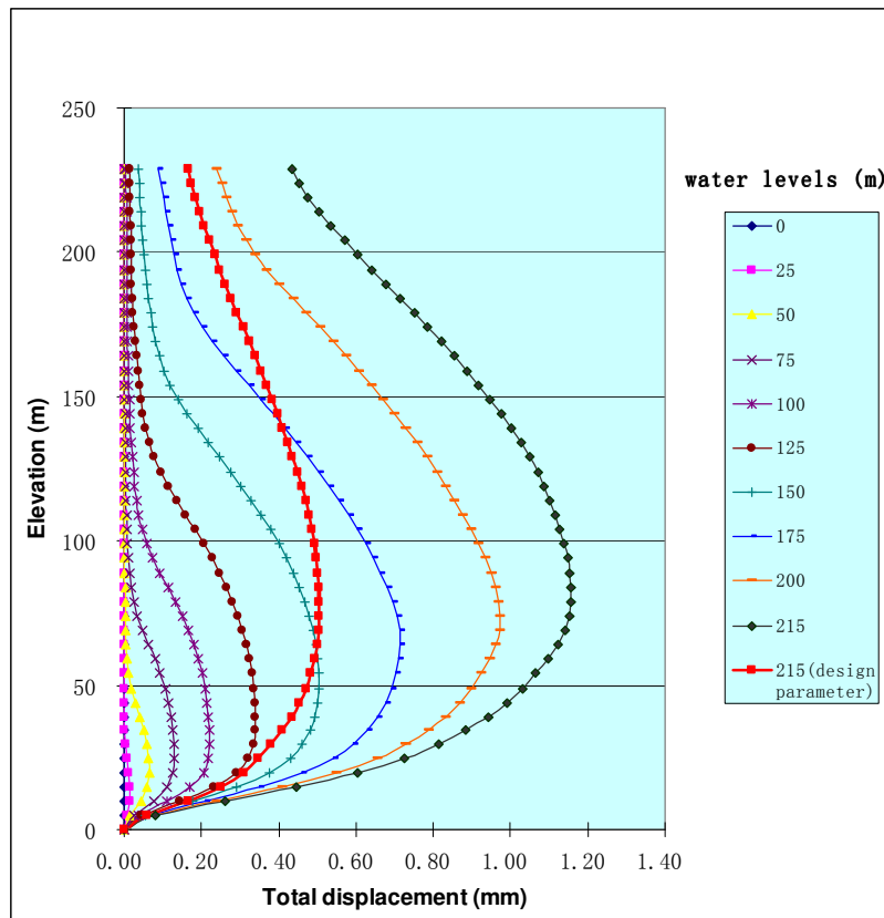
Figure 9: Total displacements (m) of the concrete face slab during the filling of the reservoir
