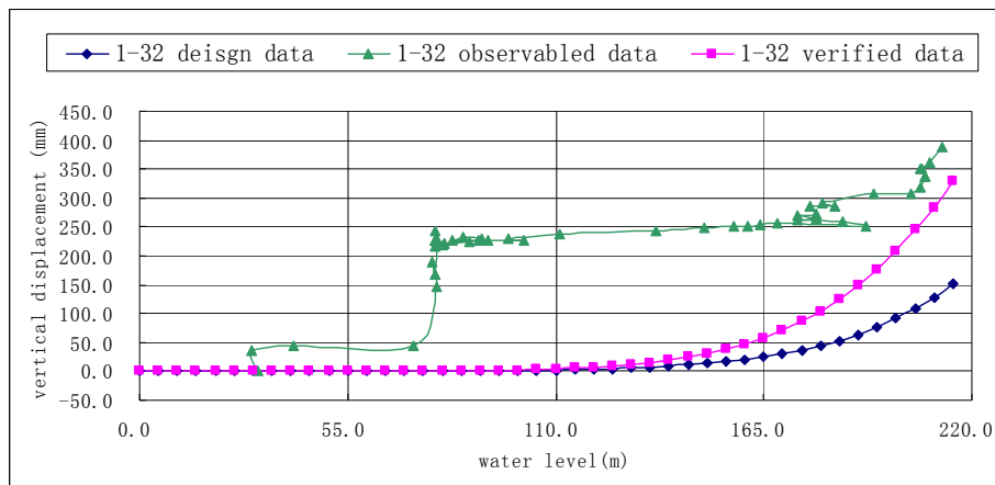
Figure 7: Settlement of pt 32.
