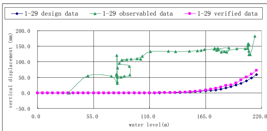
Figure 6: Settlement of pt 29.
