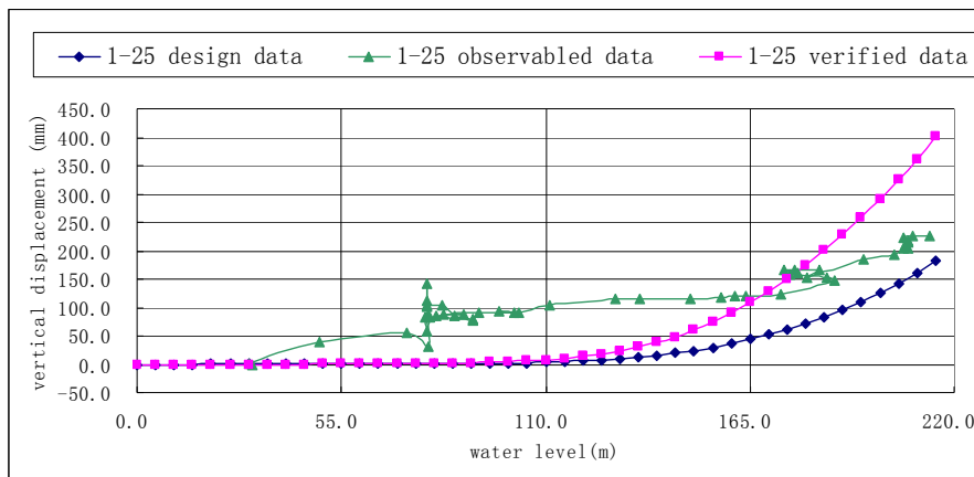
Figure 5: Settlement of pt 25.
